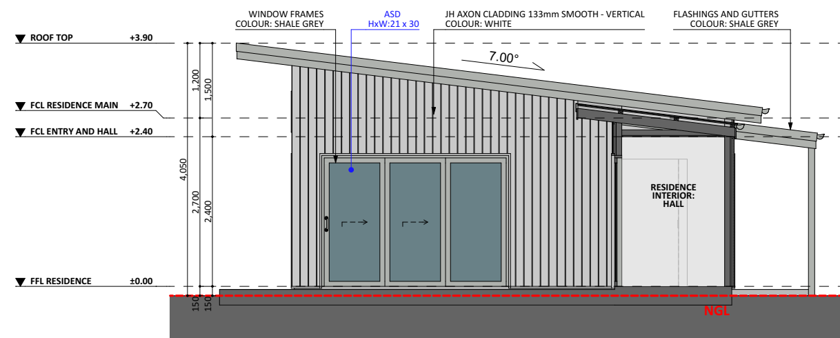
WEST ELEV. 2
