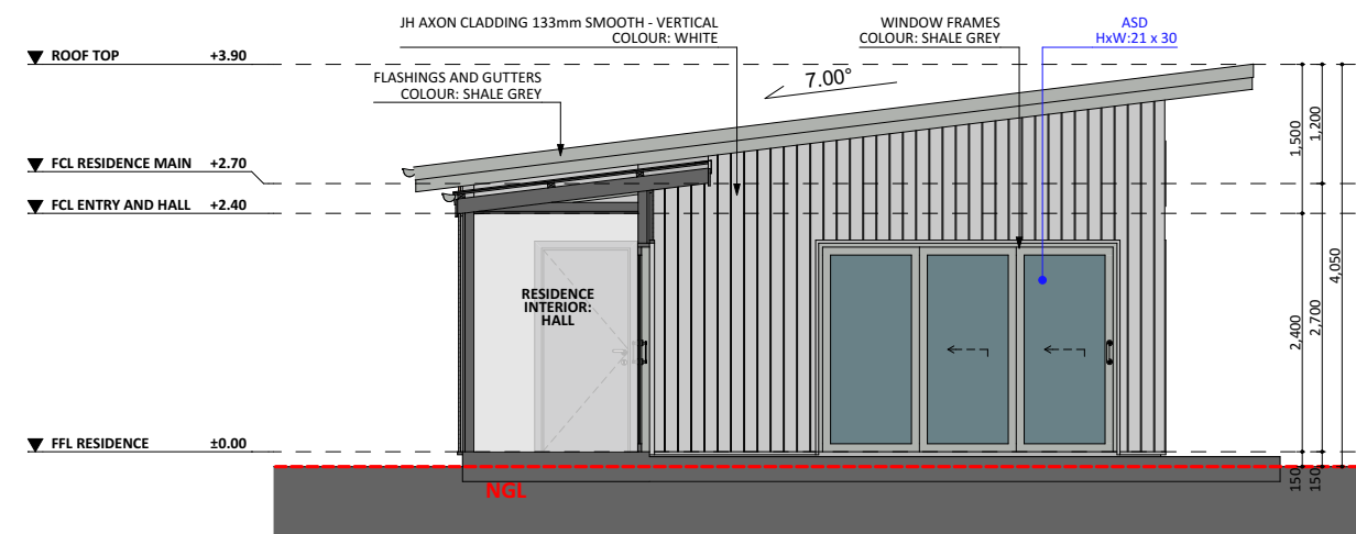
EAST ELEV. 3
