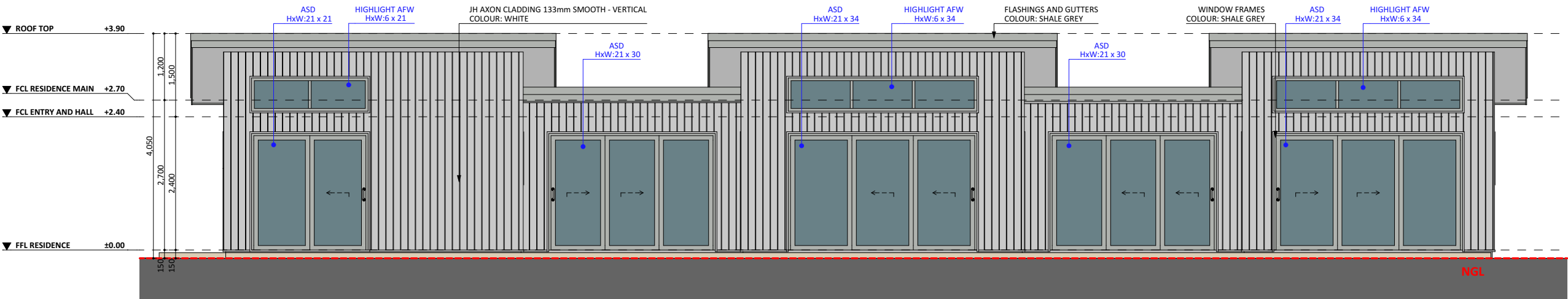
NORTH ELEV.
