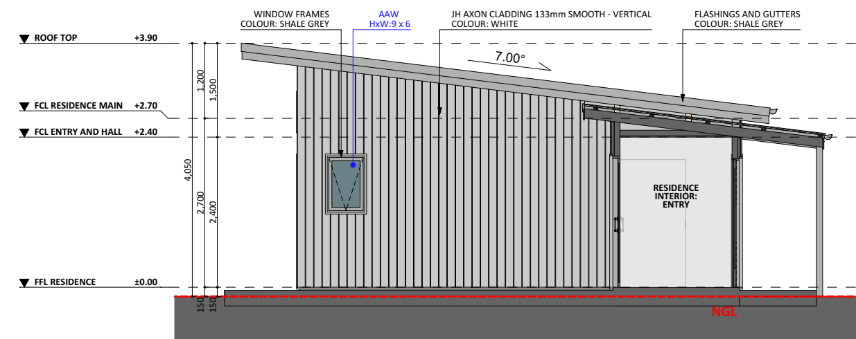
WEST ELEV. 3
