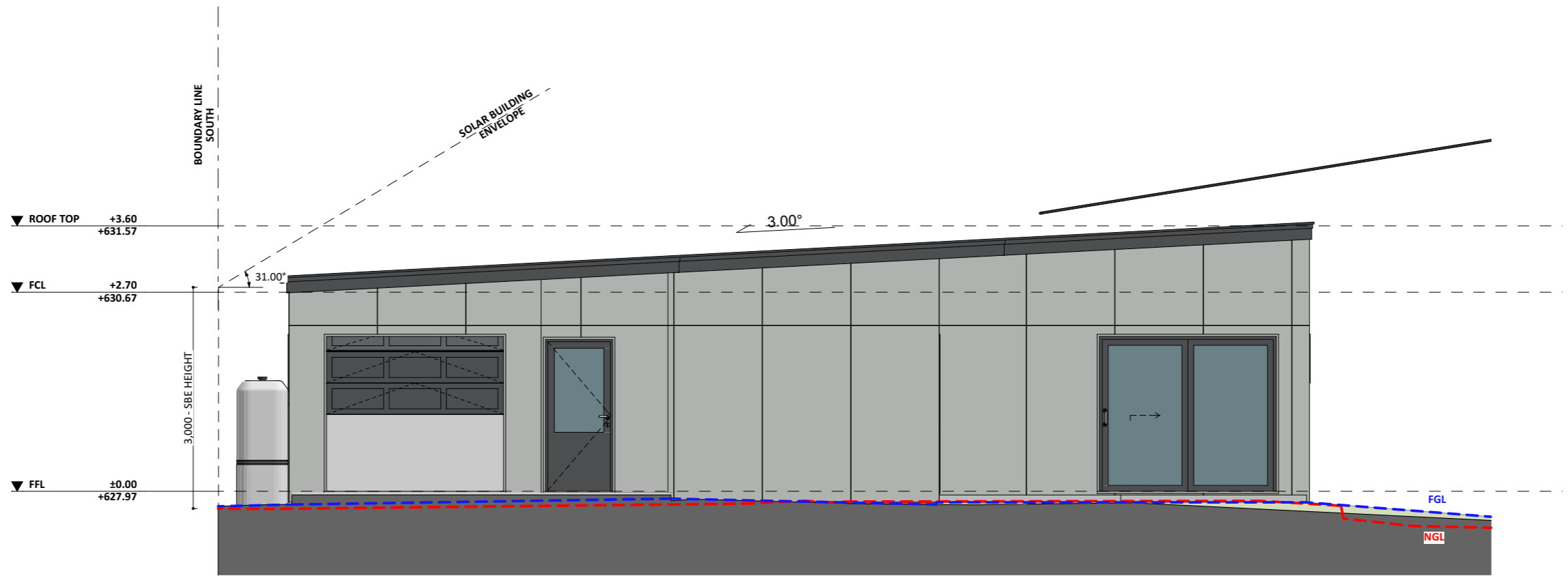
EAST ELEV.
